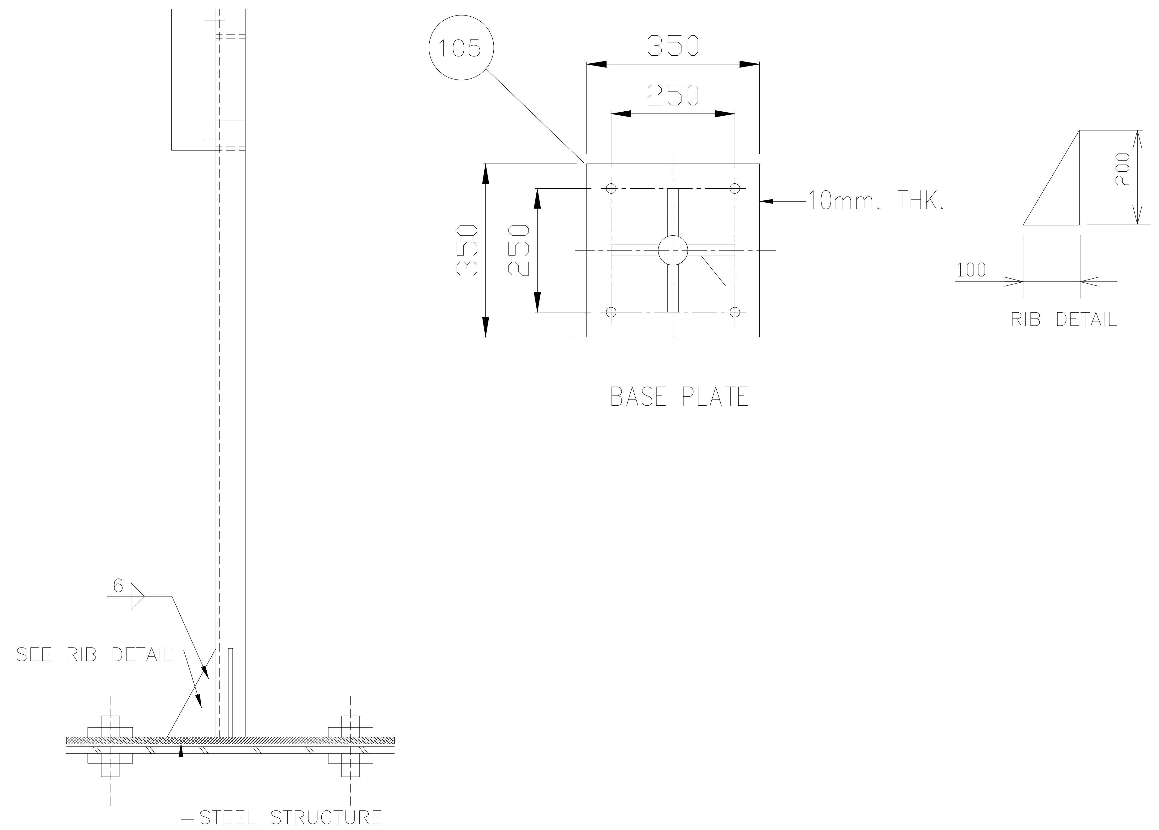
SIDE VIEW
